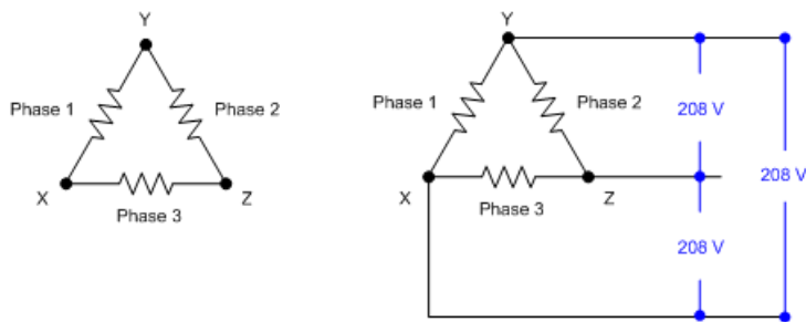
Figure 6 – North American 3-phase Delta power
