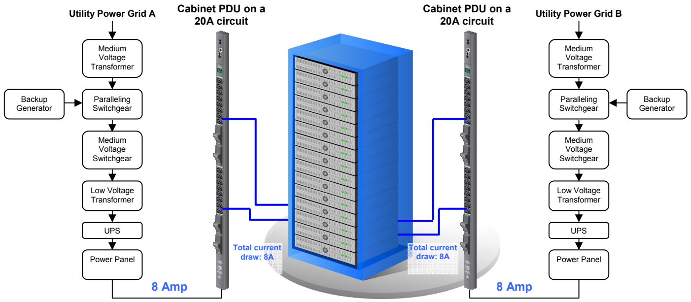
Figure 12 – Normal operation and properly loaded
