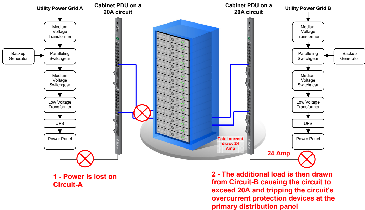
Figure 11 – A fault in Circuit-A will result in the loss of Circuit-B
