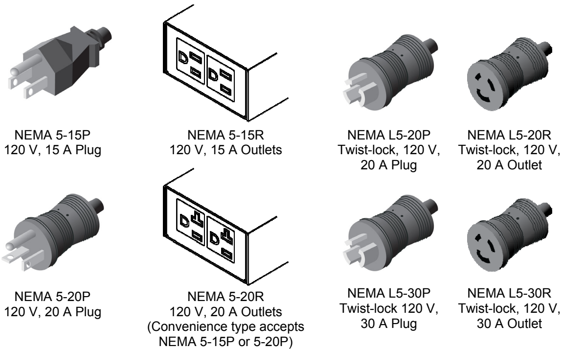
Figure 1 – Common 120 V NEMA style connectors for North America
