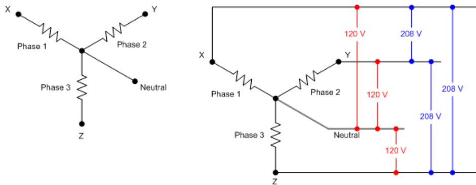
Figure 7 – North American 3-phase Wye power
