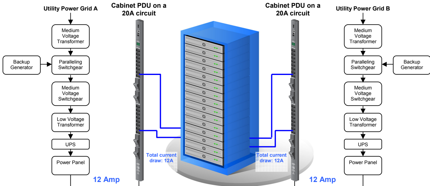
Figure 10 – Normal operation but improperly loaded
