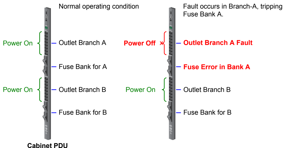
Figure 14 – Branch circuit protection
