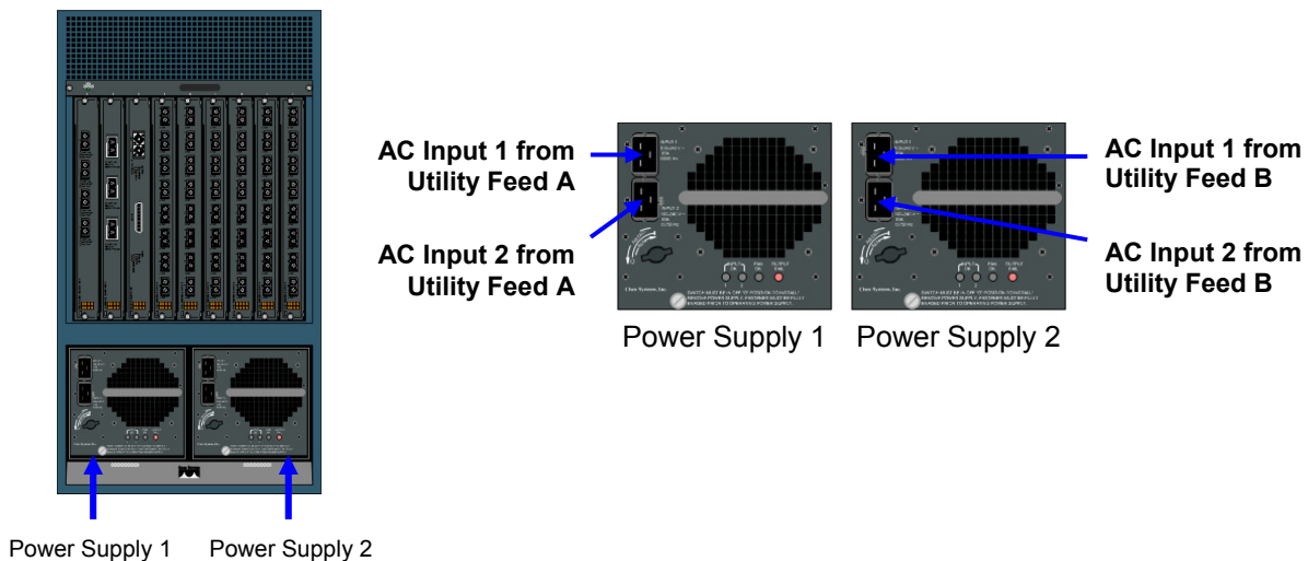
Figure 9 – The Cisco® Catalyst® Switch may be configured with two power supplies. Each supply is capable of powering the switch if the other fails. Additionally, each supply has two input power feeds that may be fed by separate and independent circuits.
