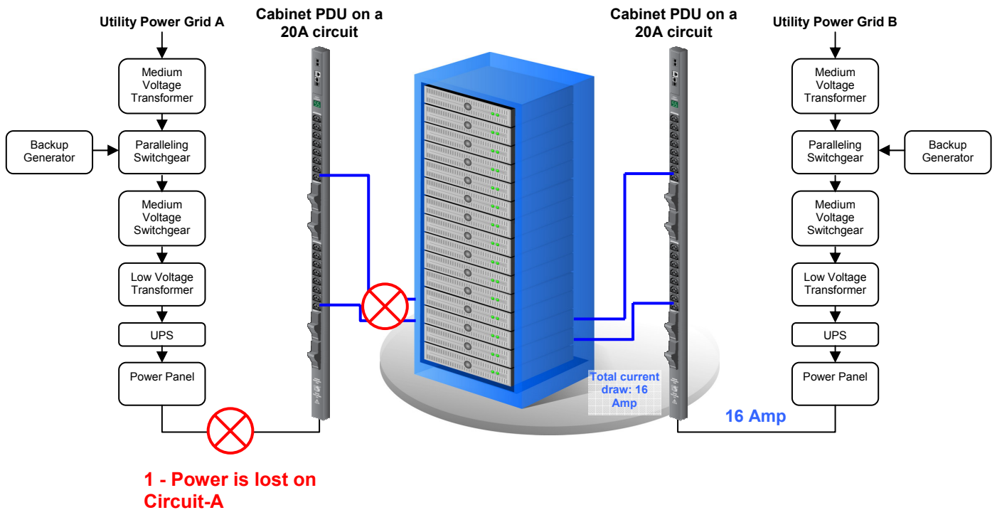
Figure 13 – Circuit-B is capable of handling the entire power load and all the equipment in the rack remains operational
