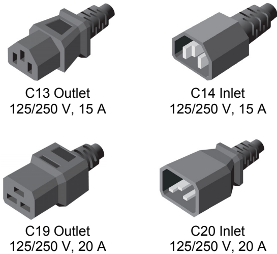
Figure 4 – Common IEC 60320 plugs and outlets
