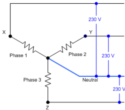
Figure 8 – International 400 V, 3-Phase Wye power
