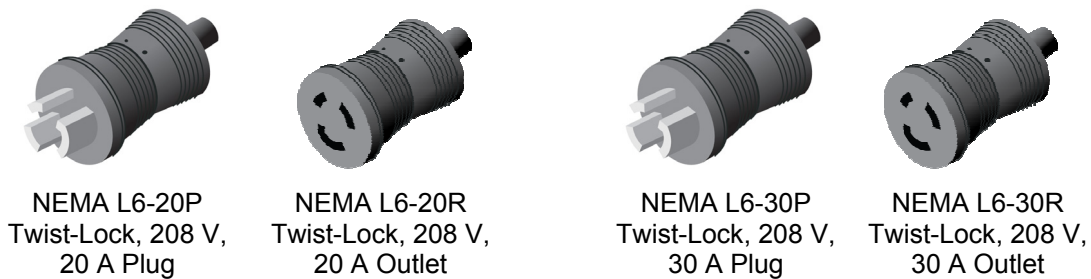
Figure 2 – Common 208 V NEMA style connectors for North America
