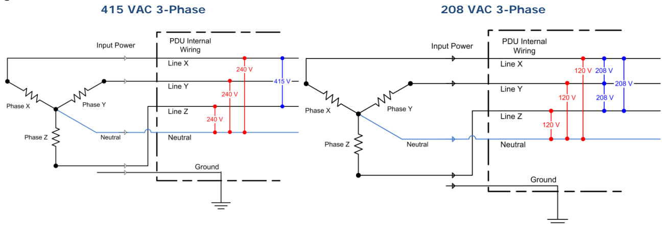
Figure 5. Difference between 415 VAC and 208 VAC power distribution systems
